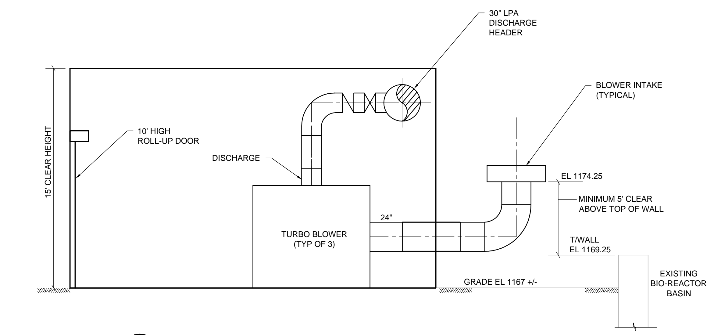
1 SECTION-BLOWER BUILDING SCALE: 1/4" = 1'-0"
